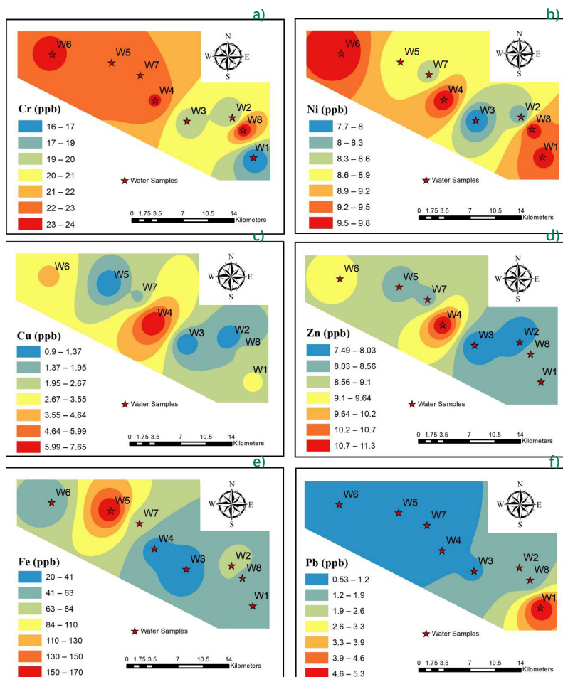
Figure 4. Spatial distribution of metal elements ( \mu\text{g/l} ) in groundwater samples of Konaro
