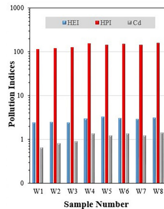
Figure 6. Comparative study of pollution evaluation indices
